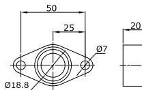
Suporte central Ref.: 1200-40Pi (Material: Nylon)
